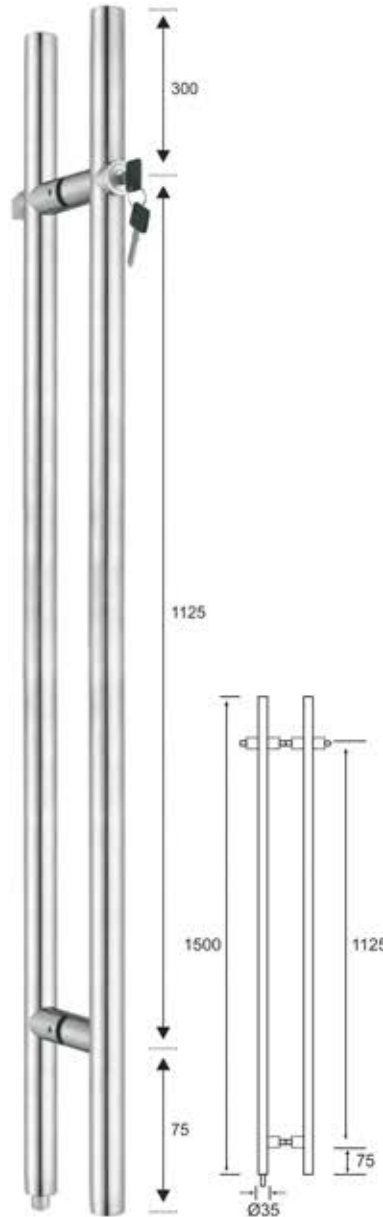
FODHL-55 Size : 35x1500mm ₹ 10800.00 Specification • Operation One side key/one side Knob • Finish : Satin stainless steel (SSS) • Material : Stainless steel 304 grade • For back to back installation • With gasket to prevent glass from damage • With grub screw to give neat look • All sizes in mm
