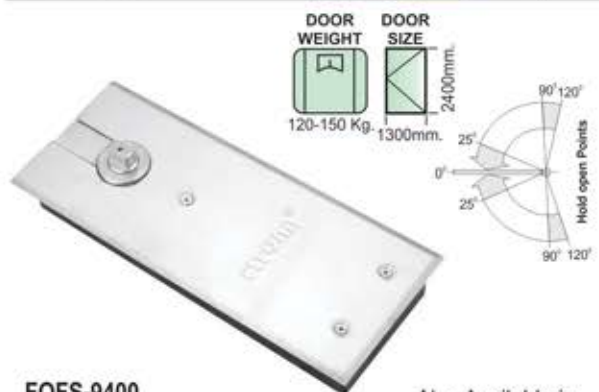
FOFS-9400 Double Spring Floor Hinge ₹ 5530.00
