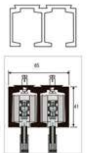
FOSL-44-B3 Aluminium Track (Double Door) Available in 8, 10 & 13 Ft. ₹ 450.00 per ft.
