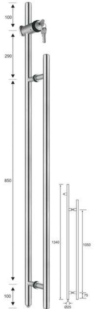
FODHL-55 Size : 25x1340mm ₹ 9900.00 Specification • Operation One side key/one side Knob • Finish : Satin stainless steel (SSS) • Material : Stainless steel 304 grade • For back to back installation • With gasket to prevent glass from damage • With grub screw to give neat look • All sizes in mm
