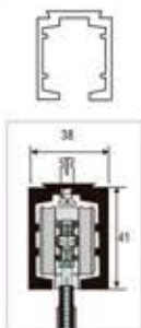
FOSL-44-B1 Aluminium Track (Single) Available in 8, 10 & 13 Ft. ₹ 270.00 per ft.
