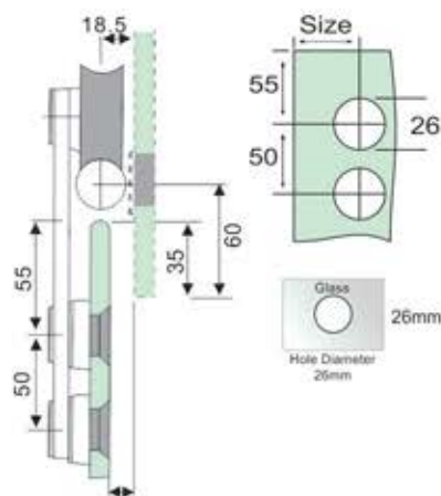
FOSL-33A Office Sliding Roller
